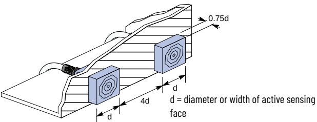
Figure 35 - Spacing Between Sensors
