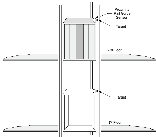
Figure 58 - Elevator Positioning
