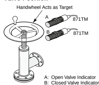
Figure 45 - Petroleum Industry – Valve Position
