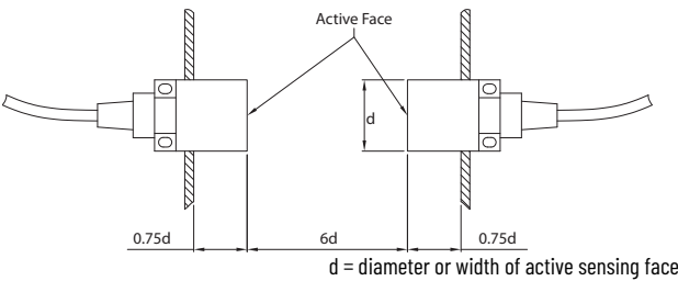
Figure 36 - Spacing Between Opposing Sensors
