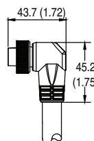
Figure B Right Angle Female
