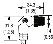
Figure H Right Angle Male
