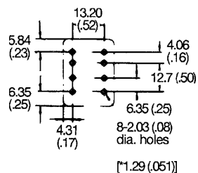
DPDT
