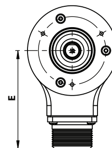
Encoder with Radial MS Connector
