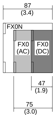
Figure: 1.1 ENG Dimensioned unit FRE Dimensions GER Abmessungen ITL Dimensioni ESP Dimensiones
