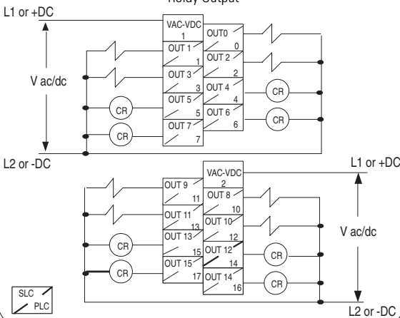
1746-OW16 Relay Output
