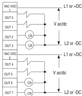
1746-OW8 Relay Output
