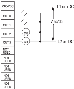
1746-OW4 Relay Output
